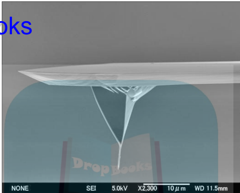
Figure 3-8: SEM image of a nanotube hanging off the tip of an AFM cantilever.
